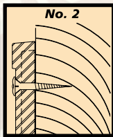
Rosettes/Wood Screws for Wood Walls
