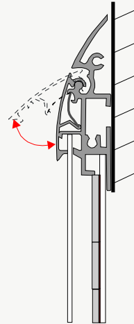
Single Sided Magnetic Directory With 1/8" Aluminum Panels
