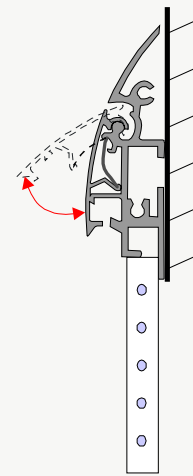
Single Sided L.E.D. Illumination
